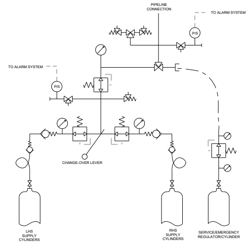
SCHEMATIC
