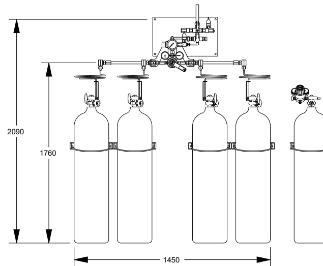
PHYSICAL
