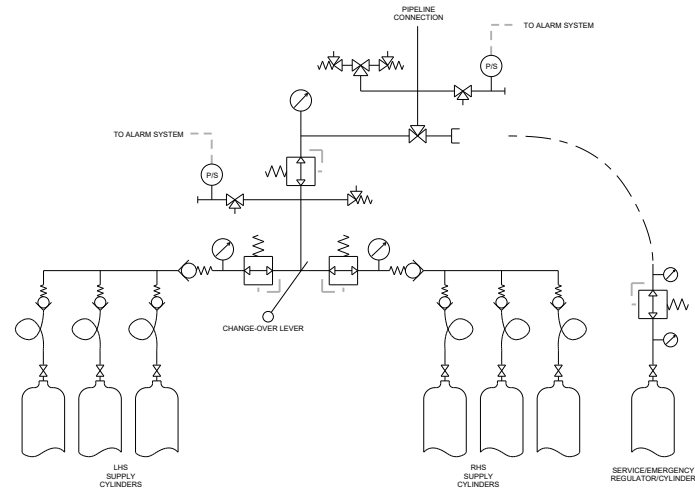
SCHEMATIC
