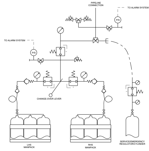
SCHMATIC
