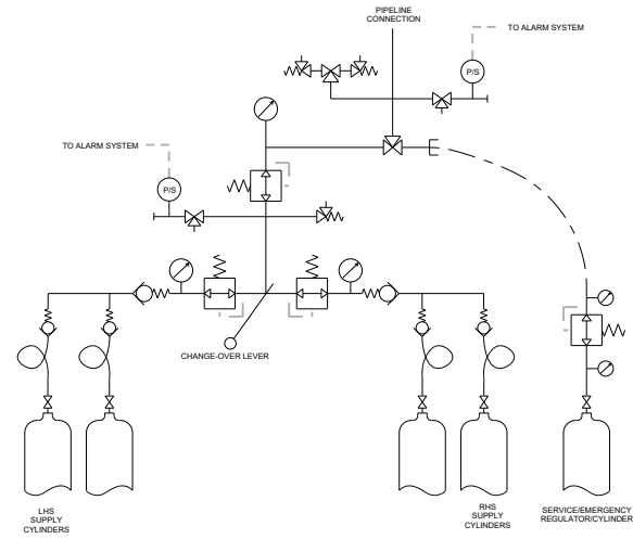
SCHEMATIC
