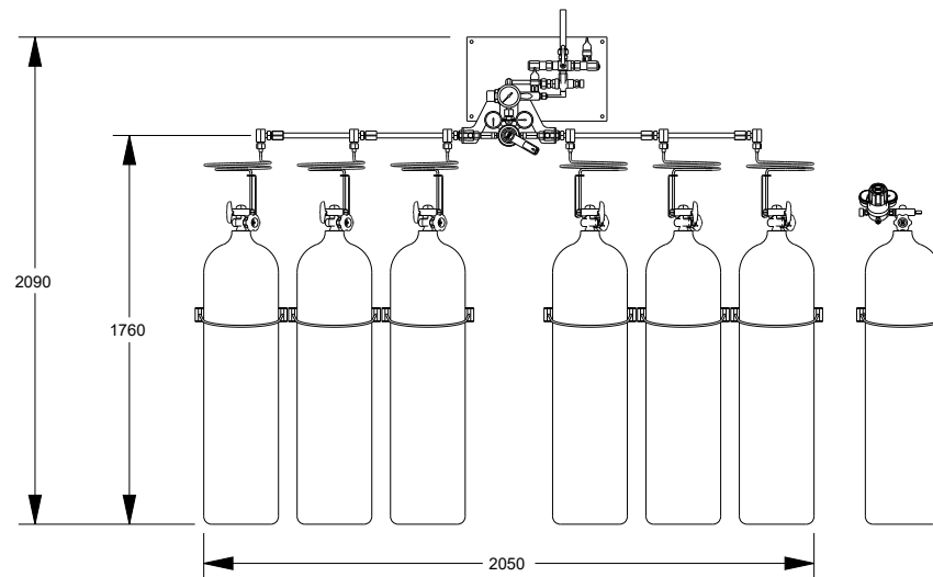
PHYSICAL
